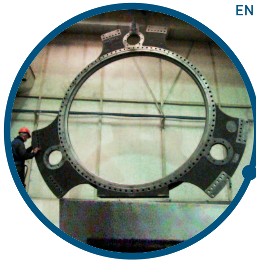
Bearing cover plate Power 5MW 4 tons EN GJS 400-18U
